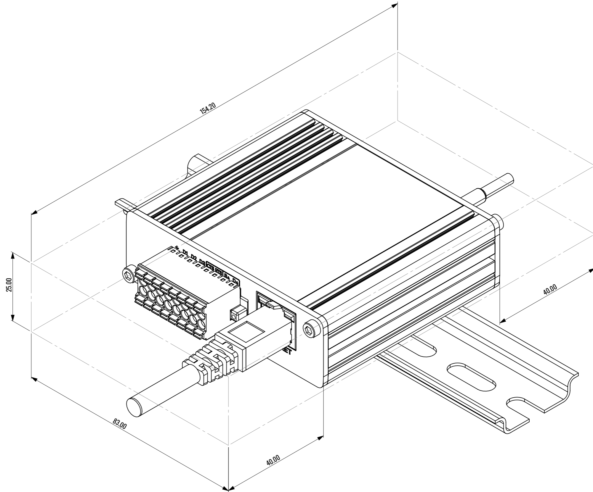
Isometric view
