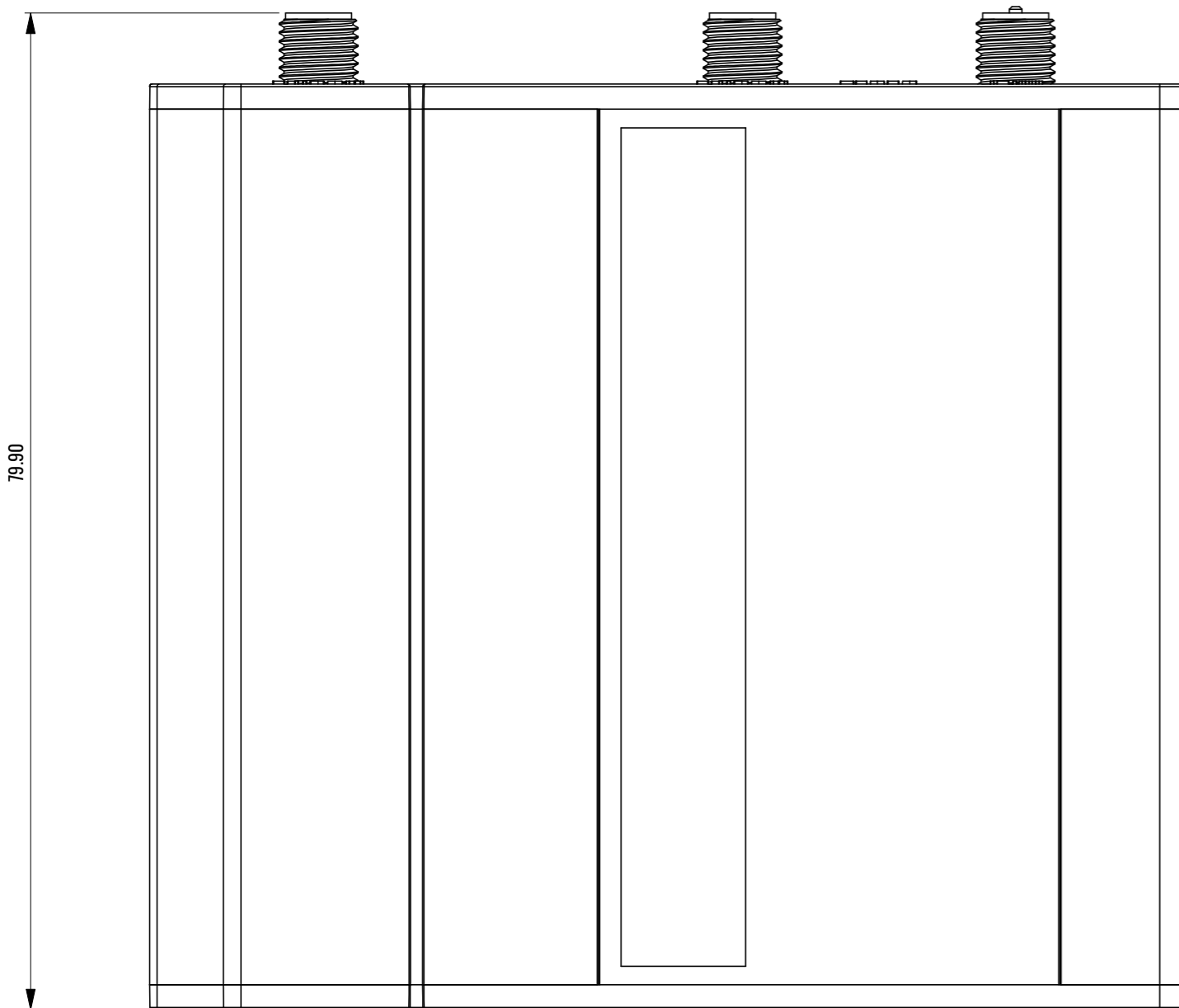
Top view
