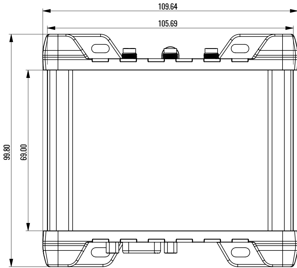
Top view
