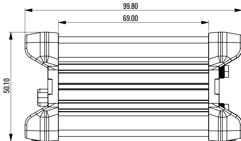
Right view
