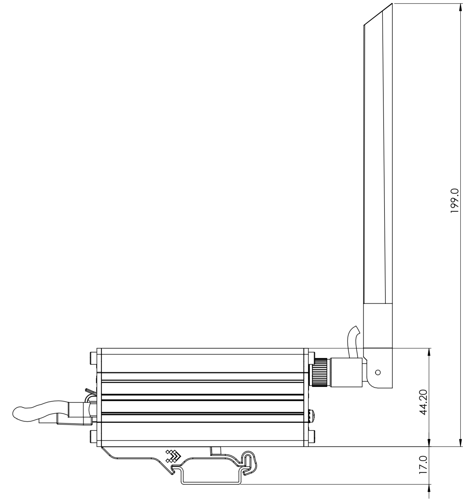
Mounting space requirements
