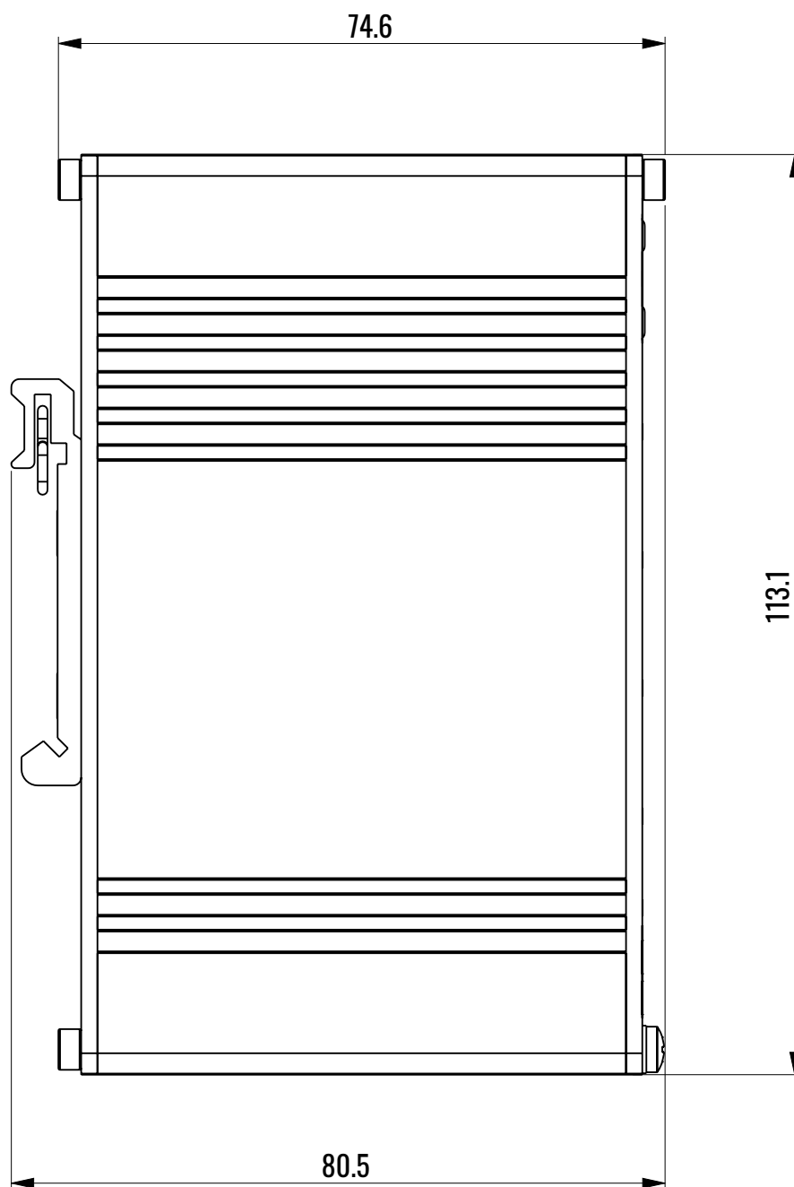
Top view
