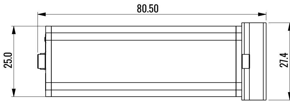
Right view
