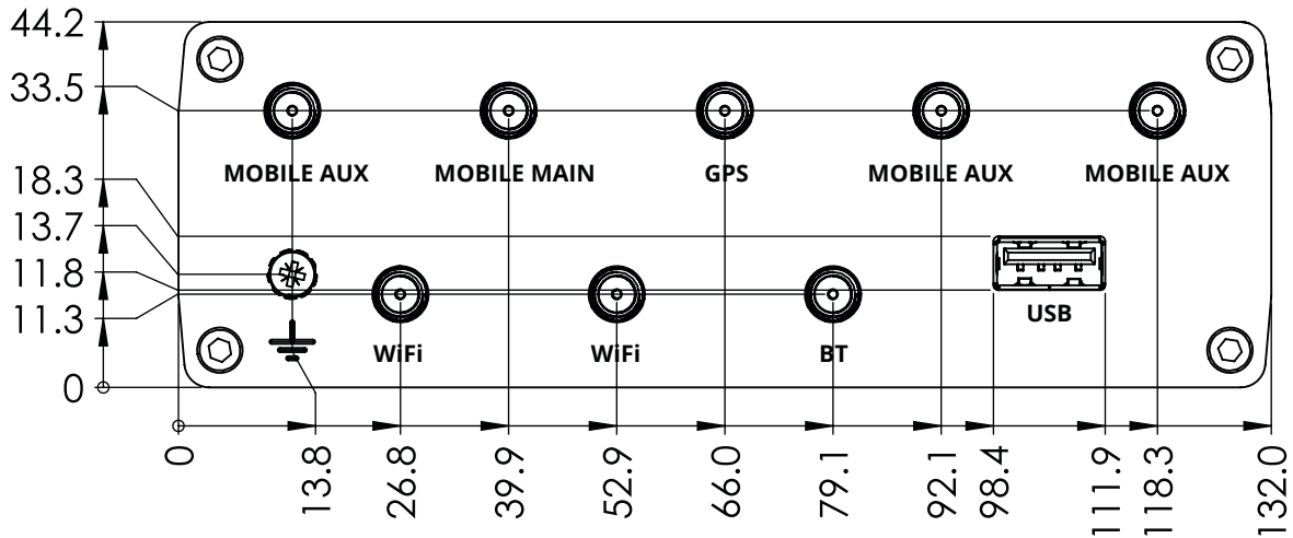
Rear view
