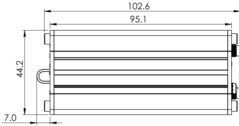
Right view
