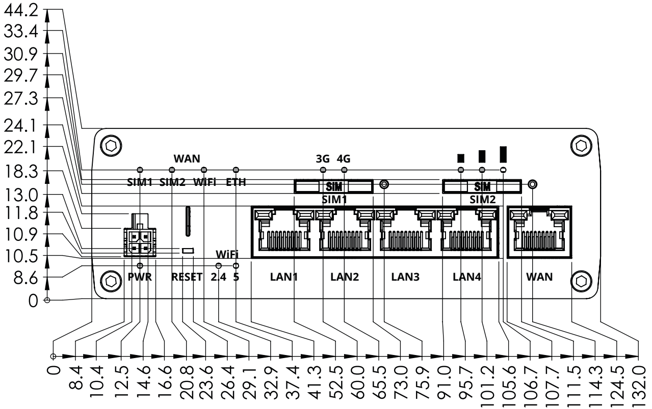
Front view
