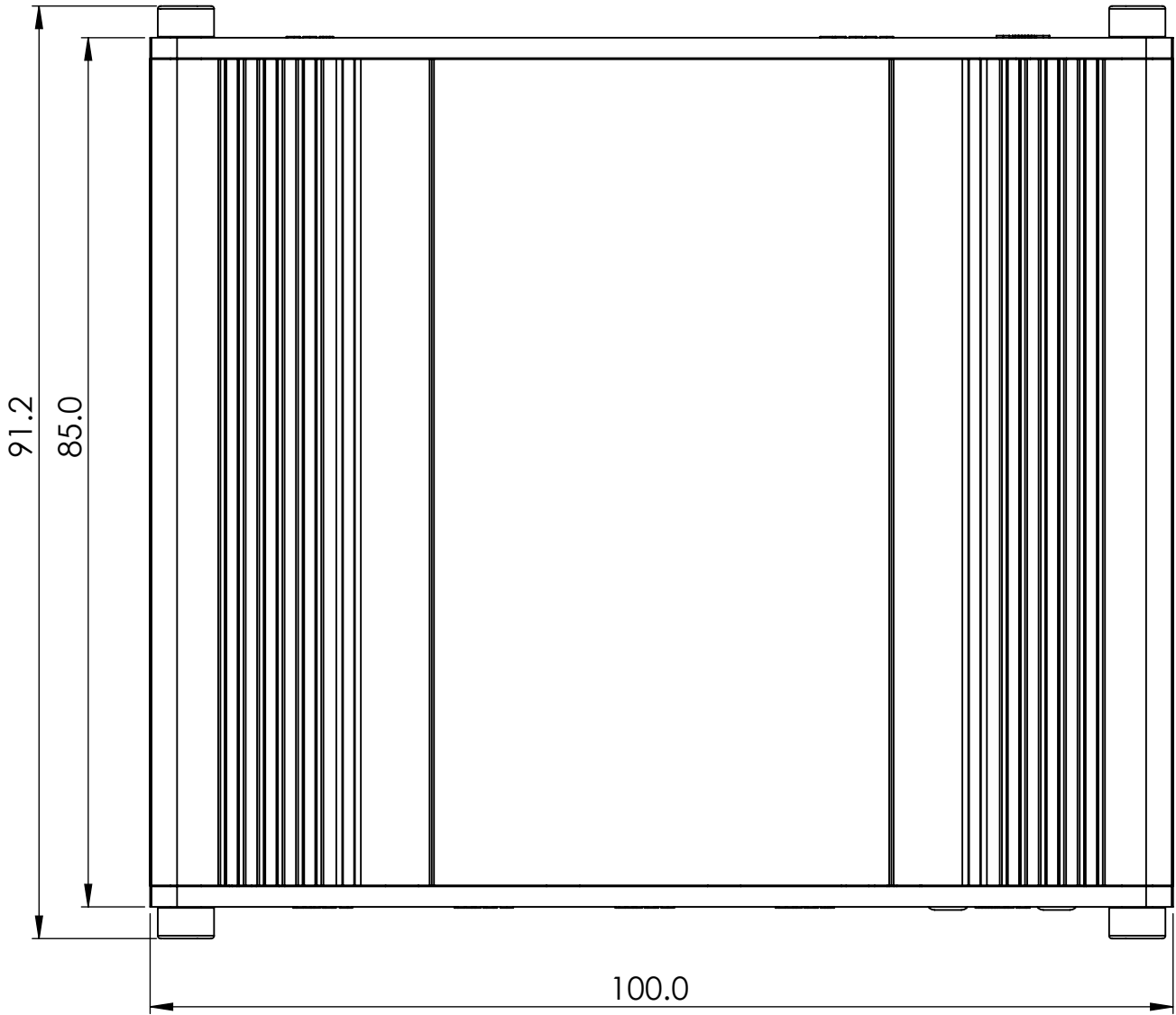
TOP view
