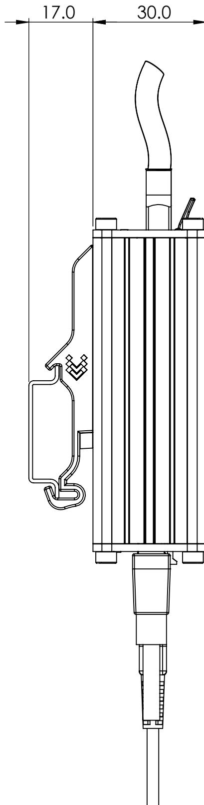
Mounting space requirements
