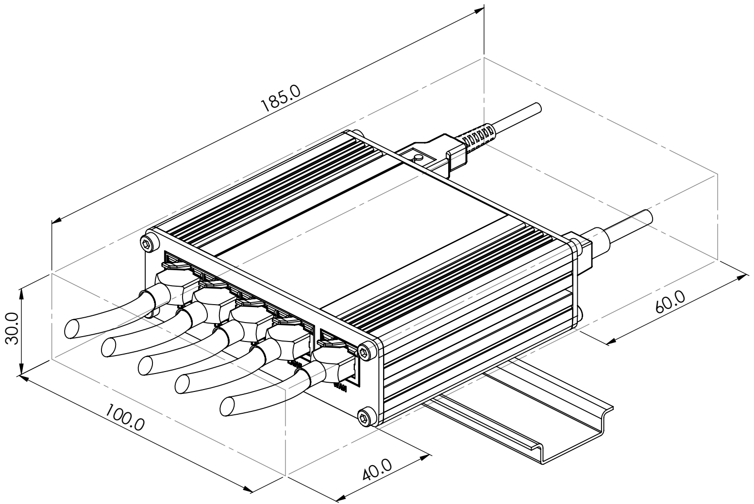
Mounting space requirements
