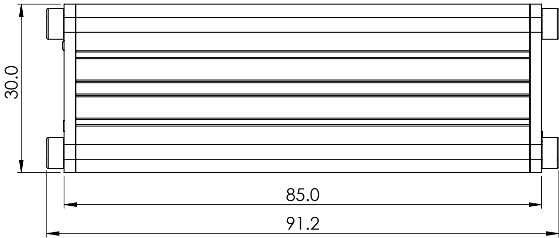
Right view
