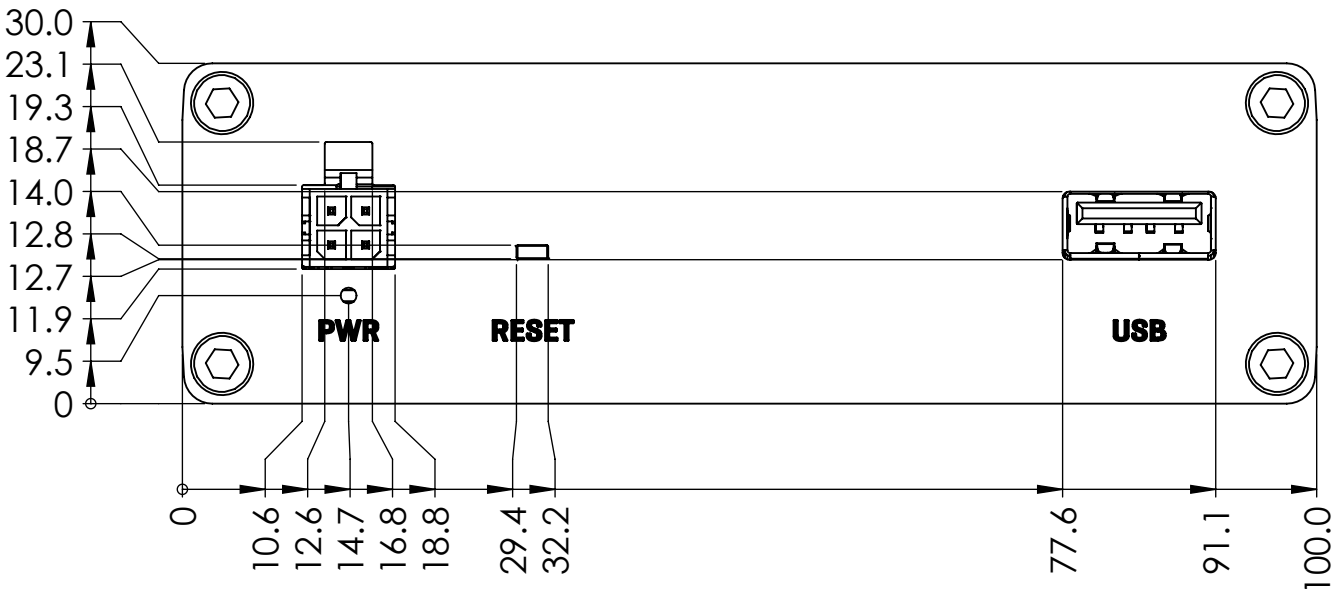
Rear view
