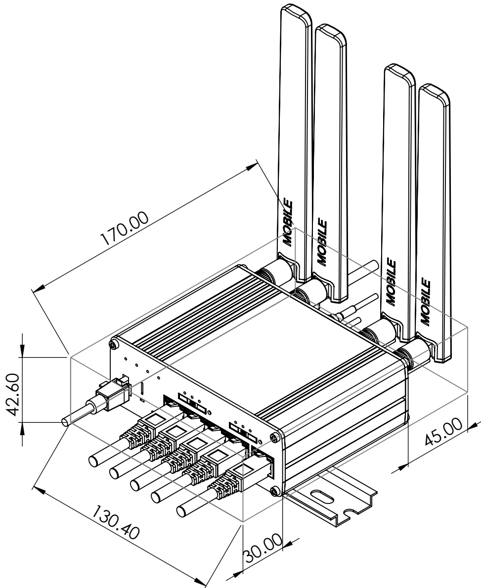
Mounting space requirements
