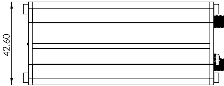
Right view
