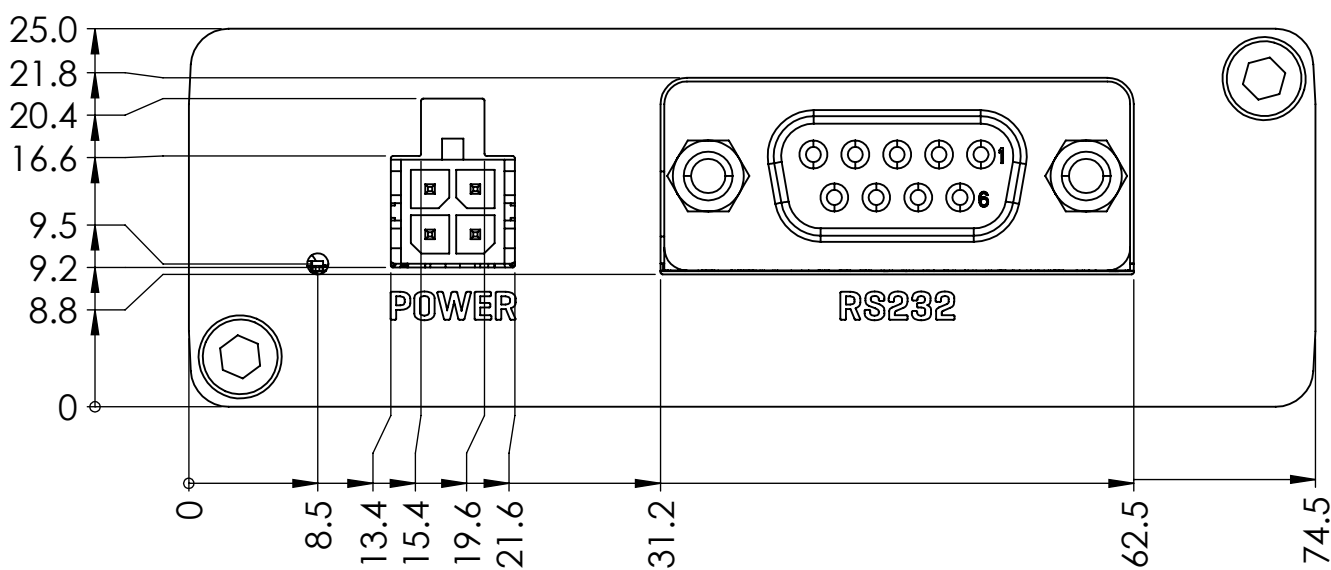
Front view
