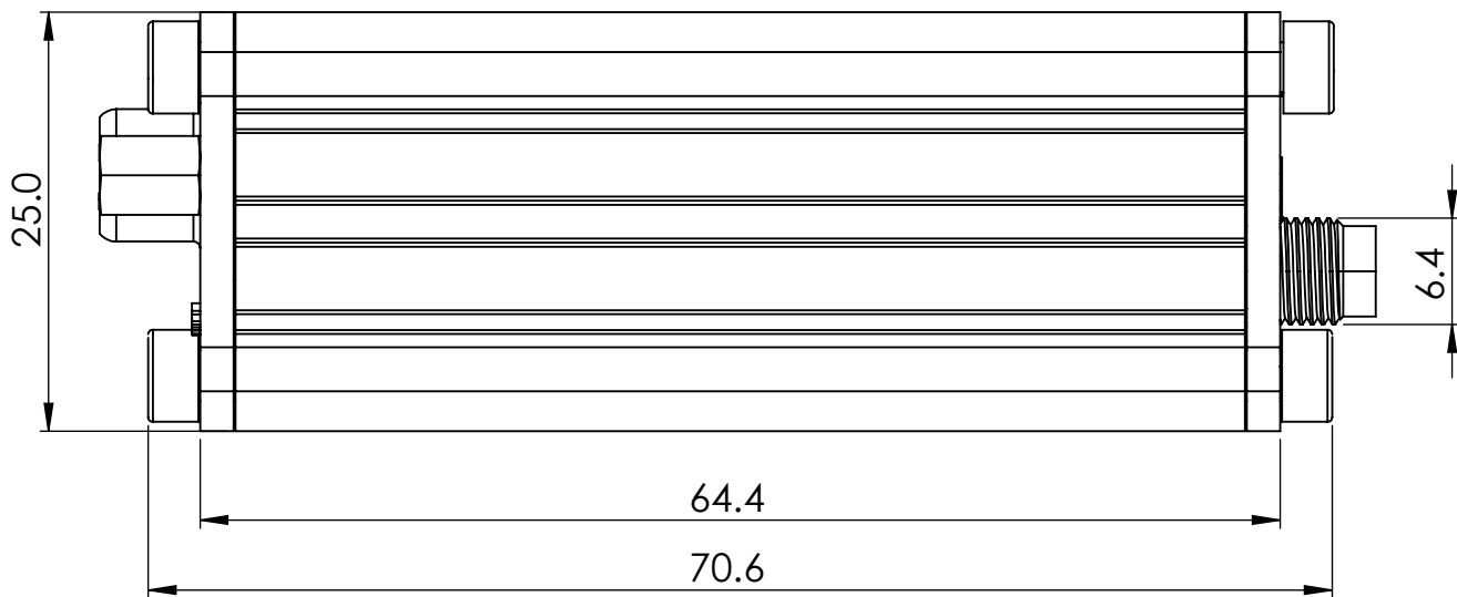
Right view
