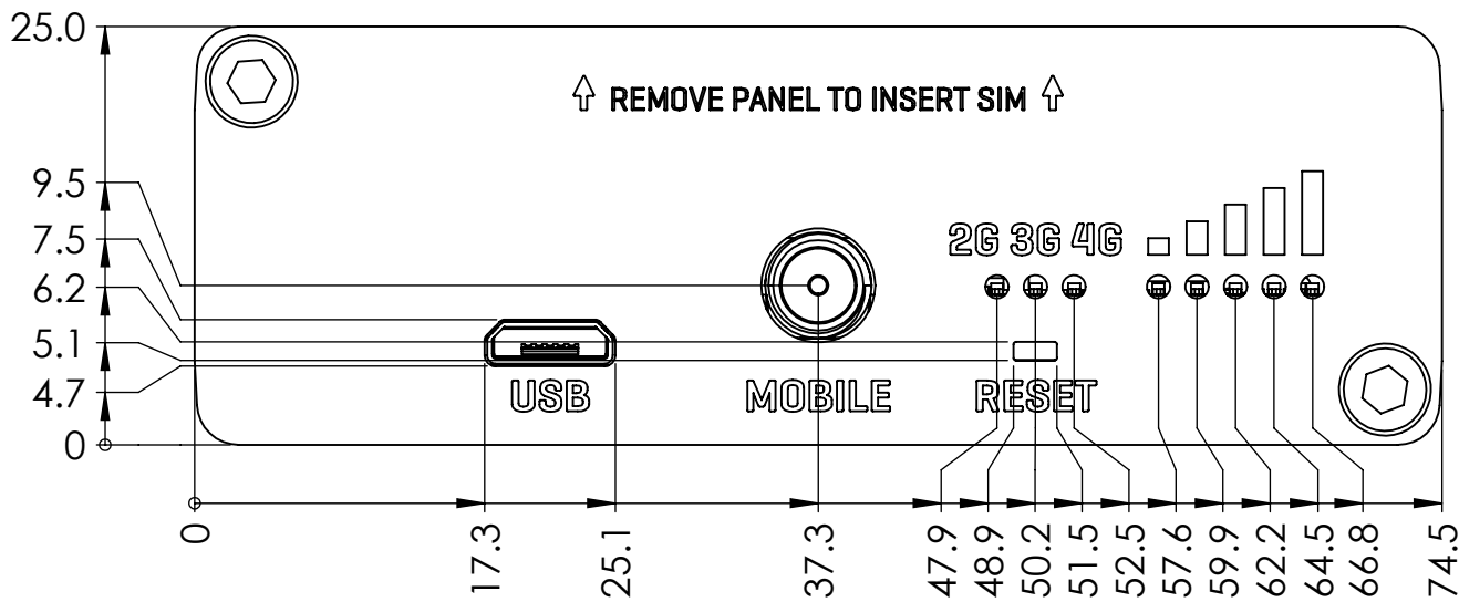
Rear view
