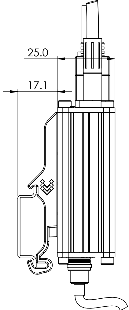
Mounting space requirements
