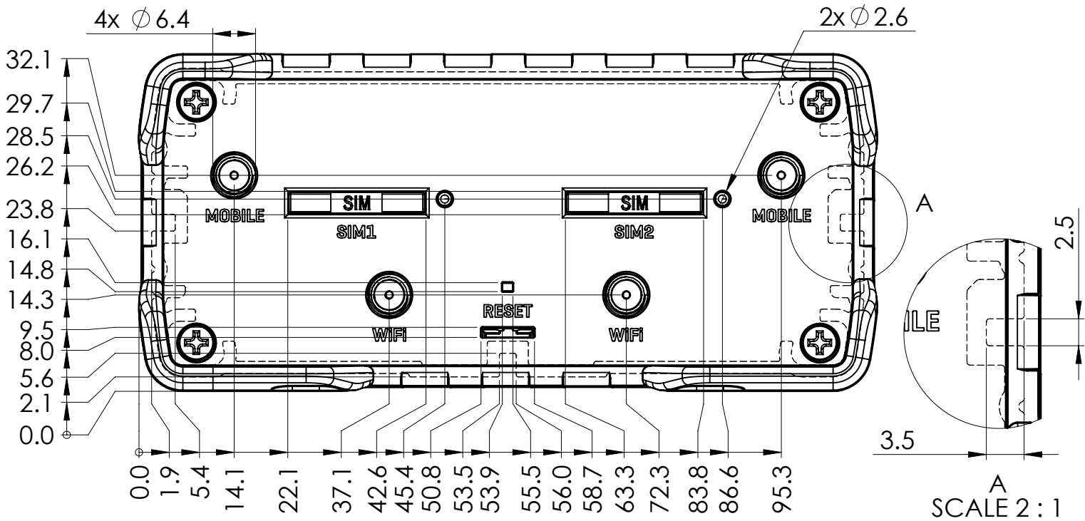
Rear view
