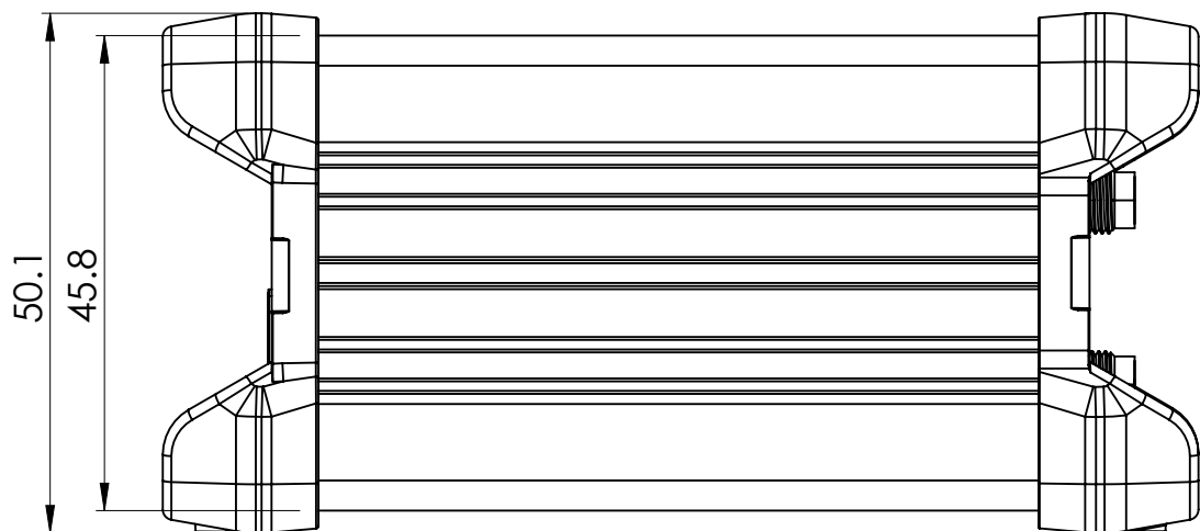
Right view
