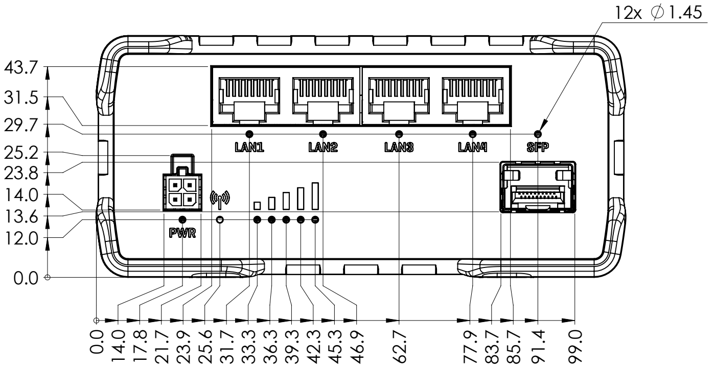
Front view
