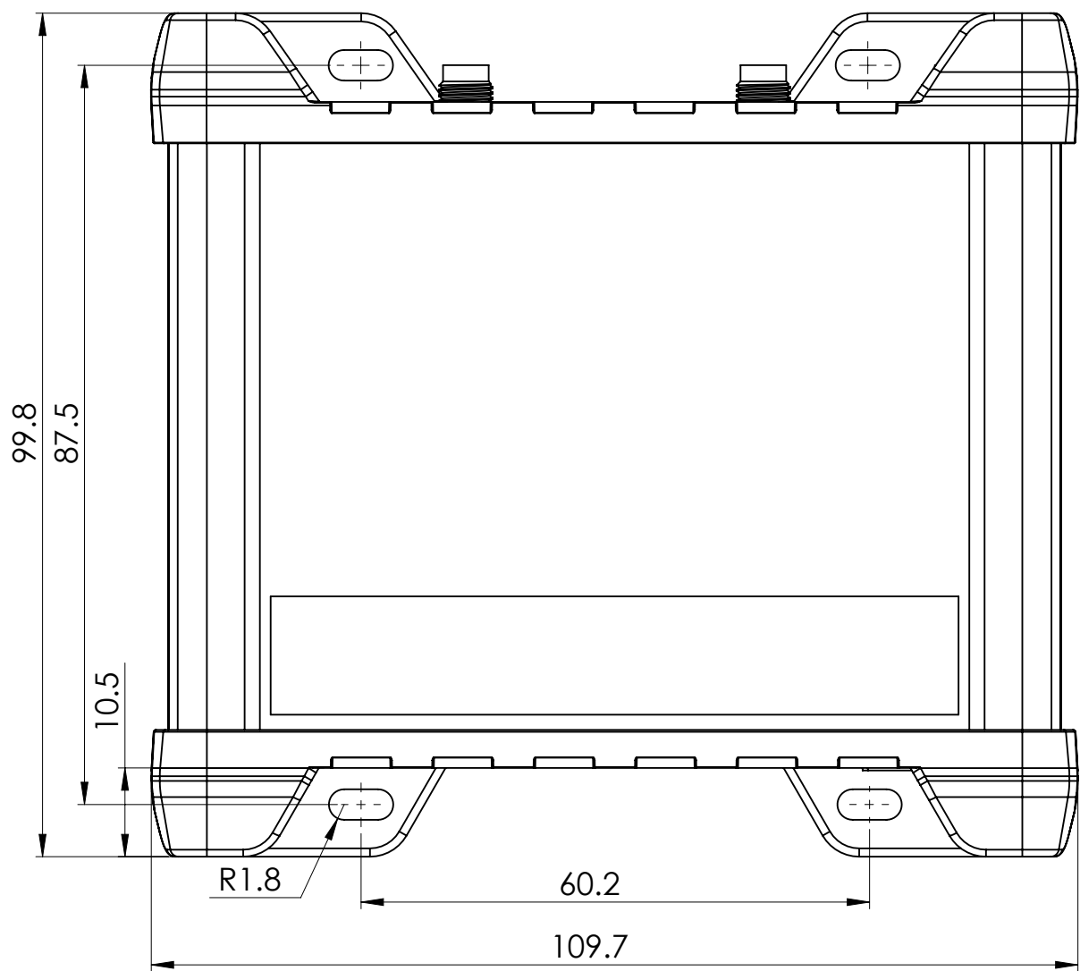
Top view
