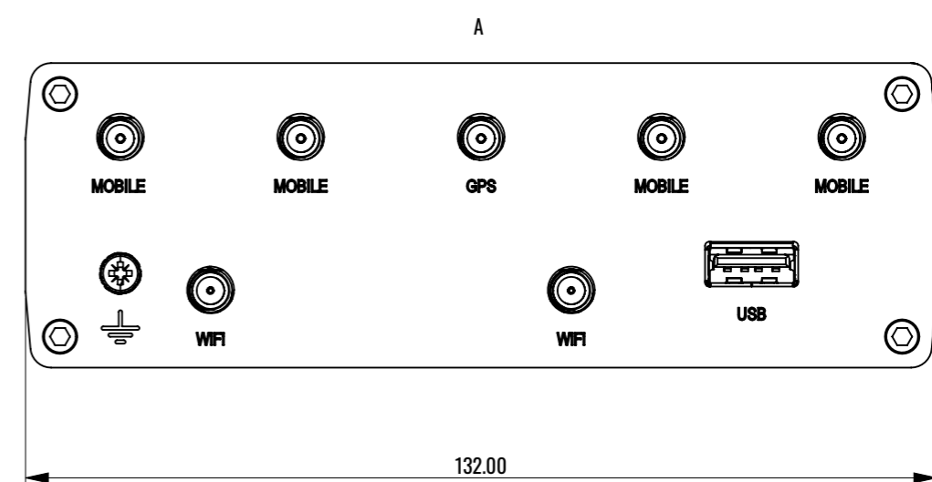
Rear view
