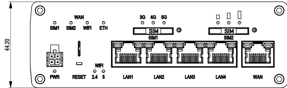
Front view
