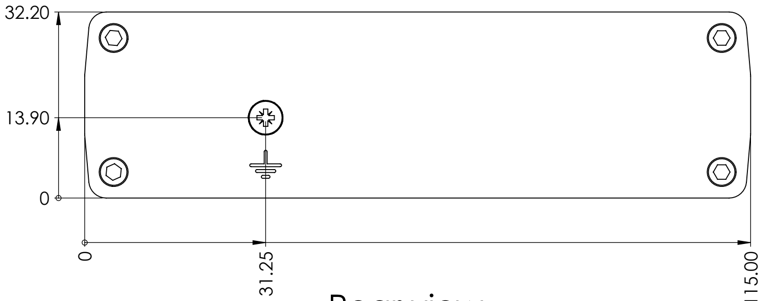
Rear view
