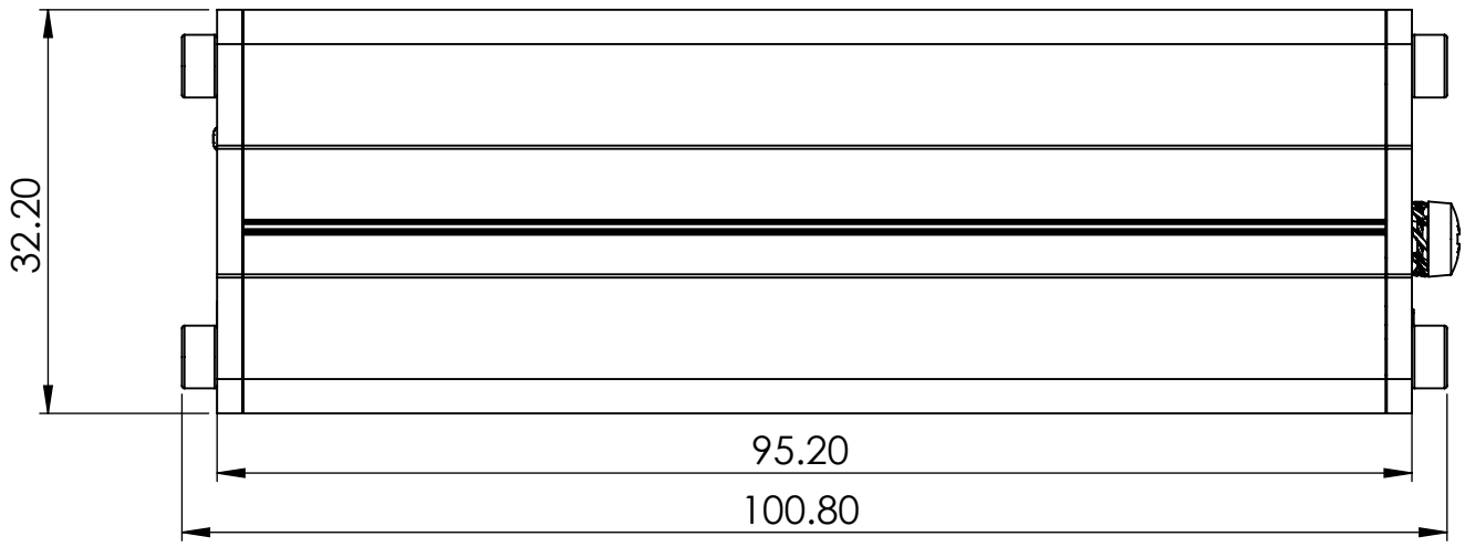
Right view
