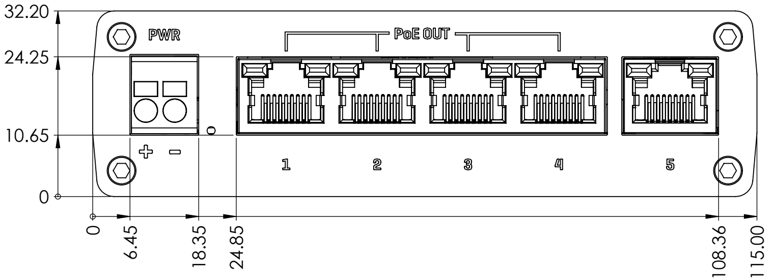
Front view
