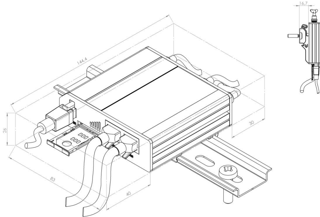
Mounting space requirements
