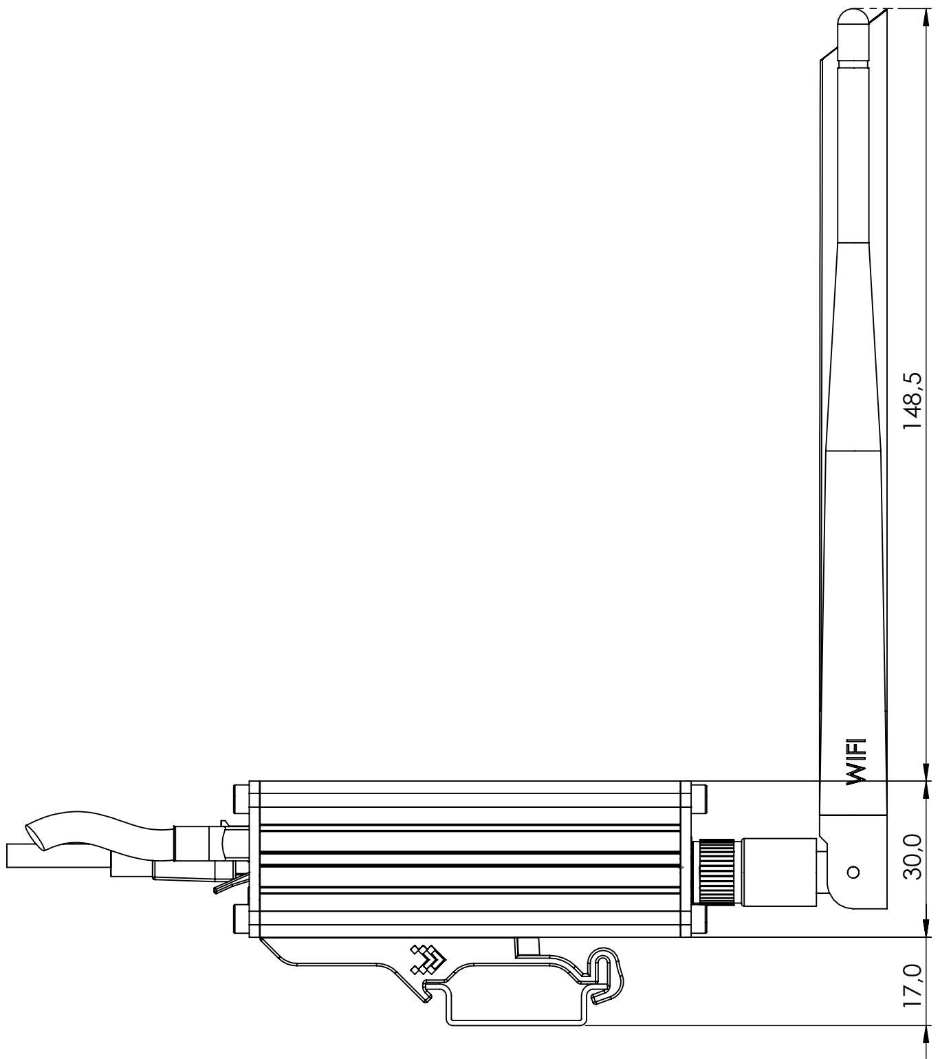
Mounting space requirements
