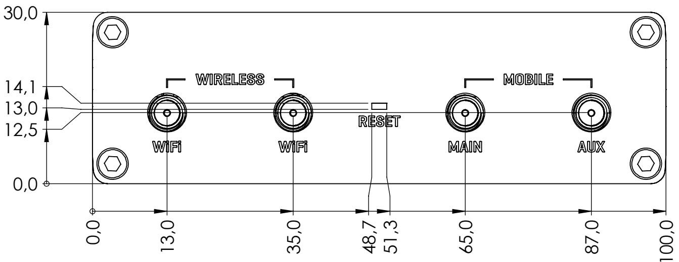
Rear view
