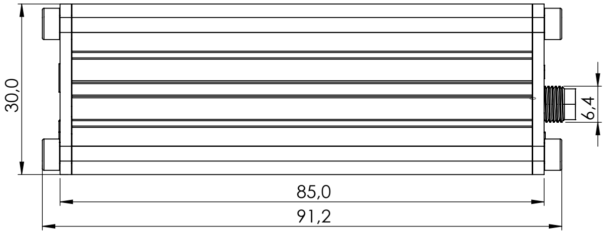
Right view
