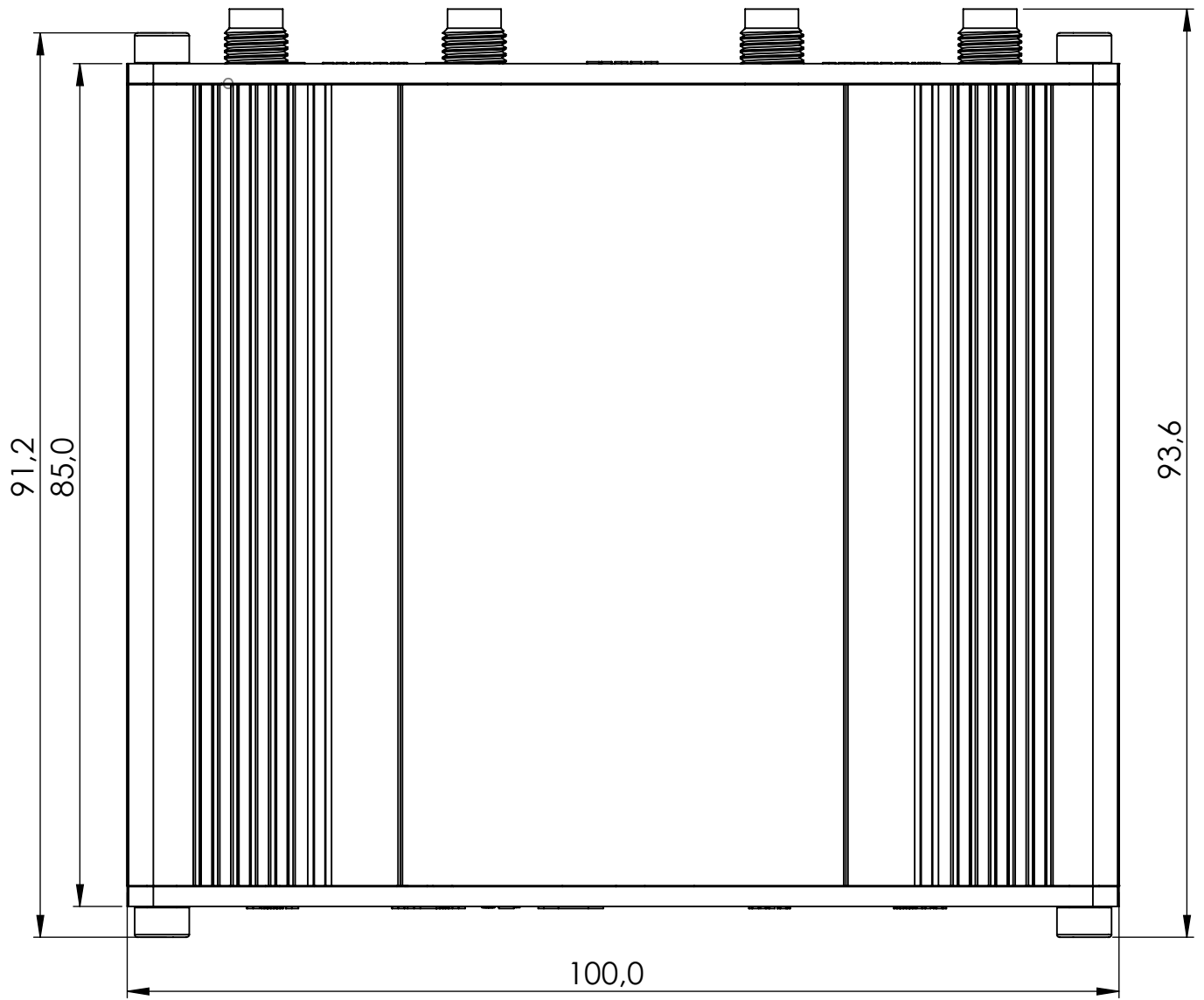
TOP view
