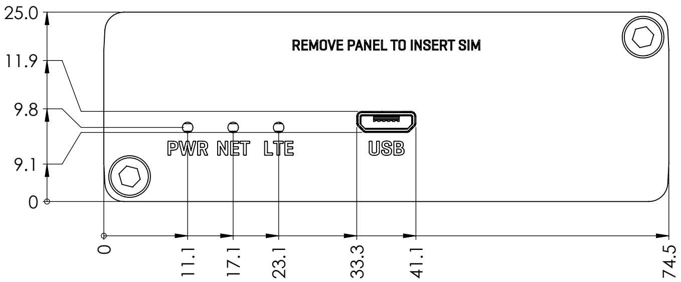
Front view
