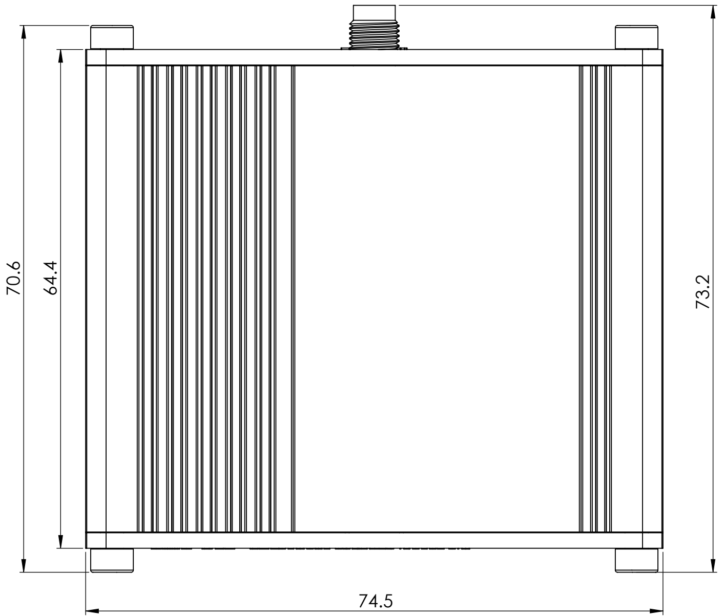
Top view
