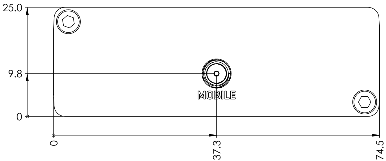
Rear view
