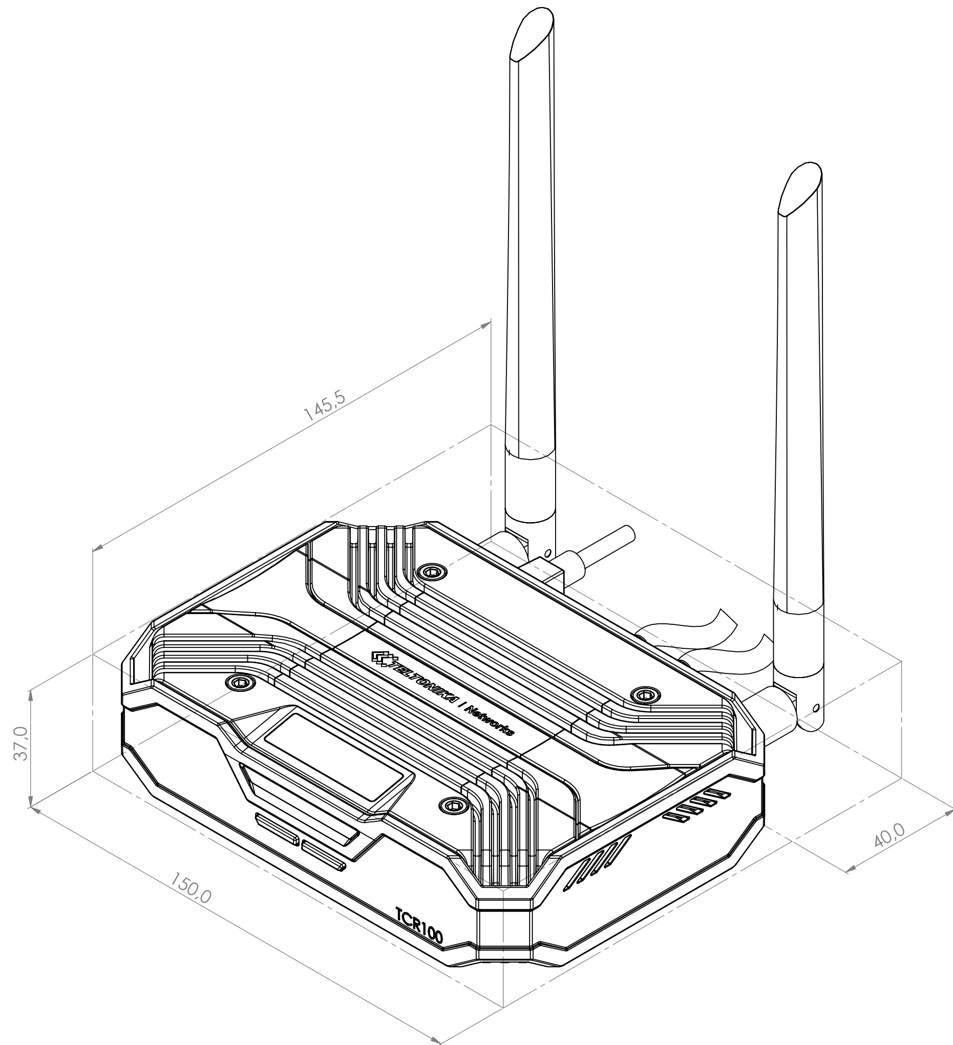
Mounting space requirements
