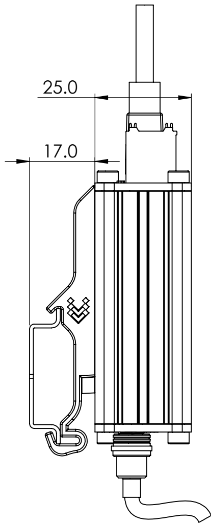
Mounting space requirements
