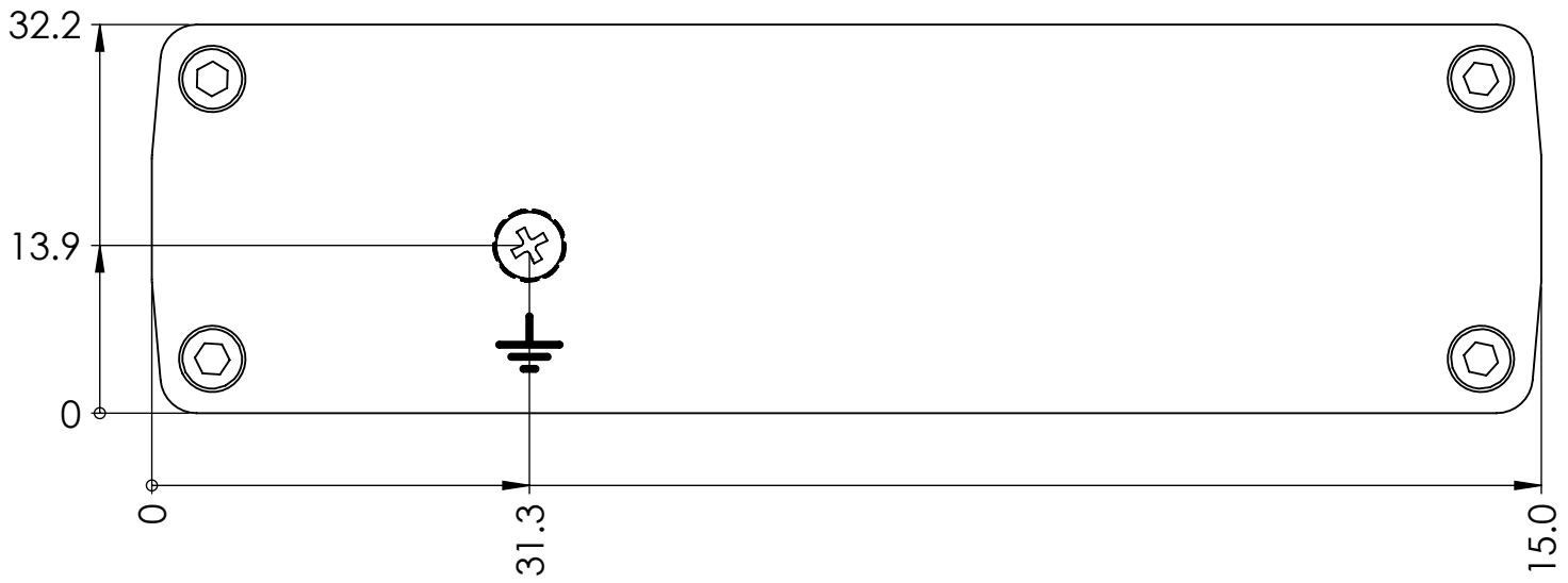
Rear view
