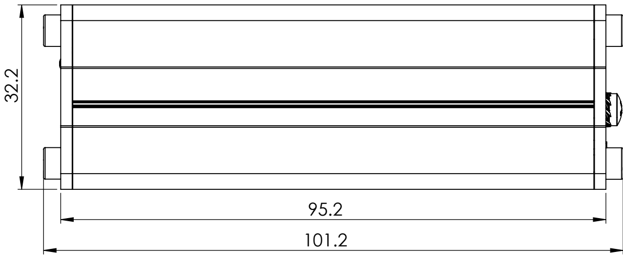
Right view
