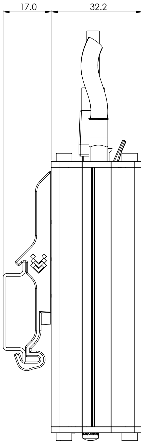
Mounting space requirements
