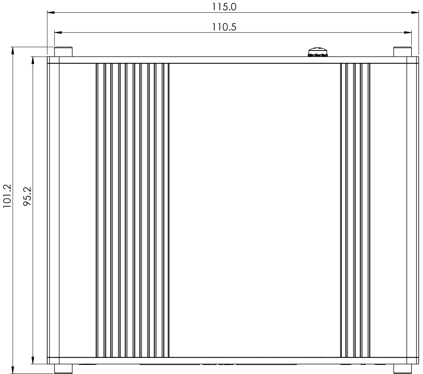
Top view
