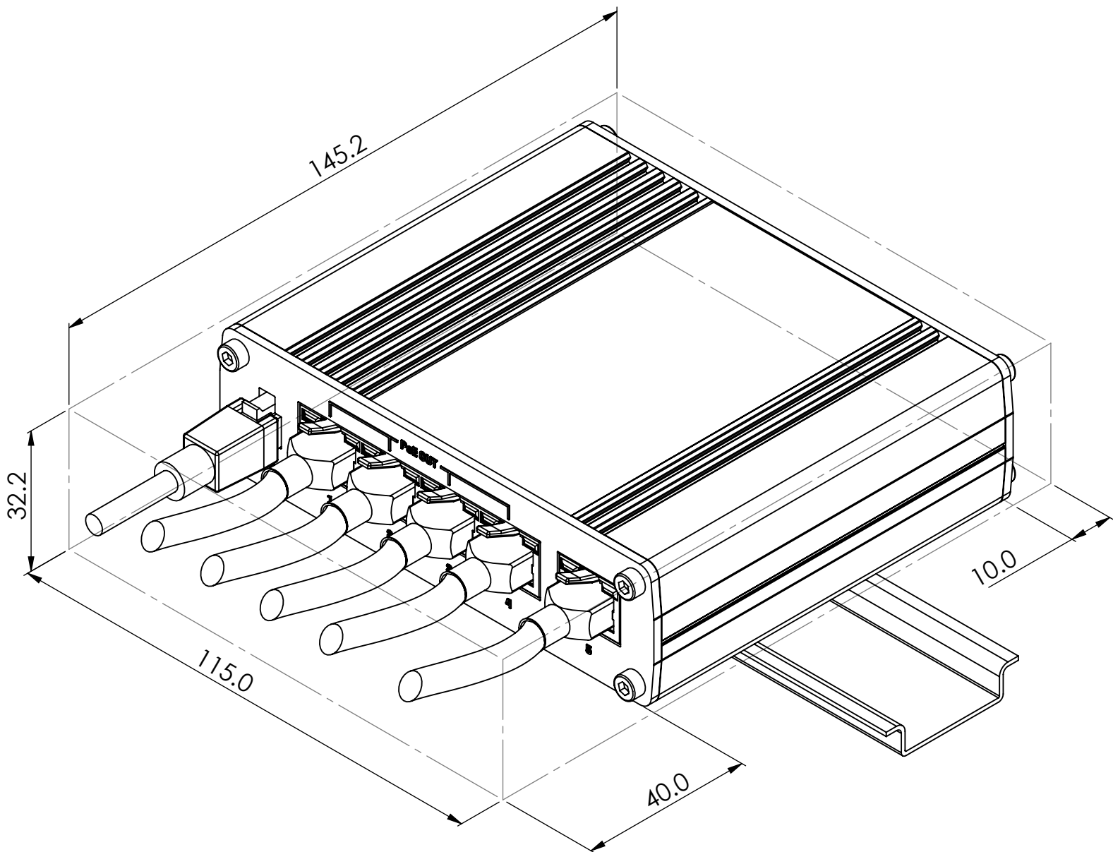
Mounting space requirements
