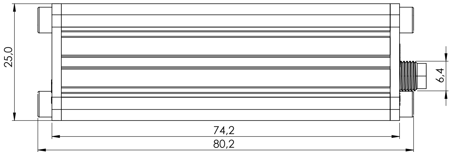
Right view
