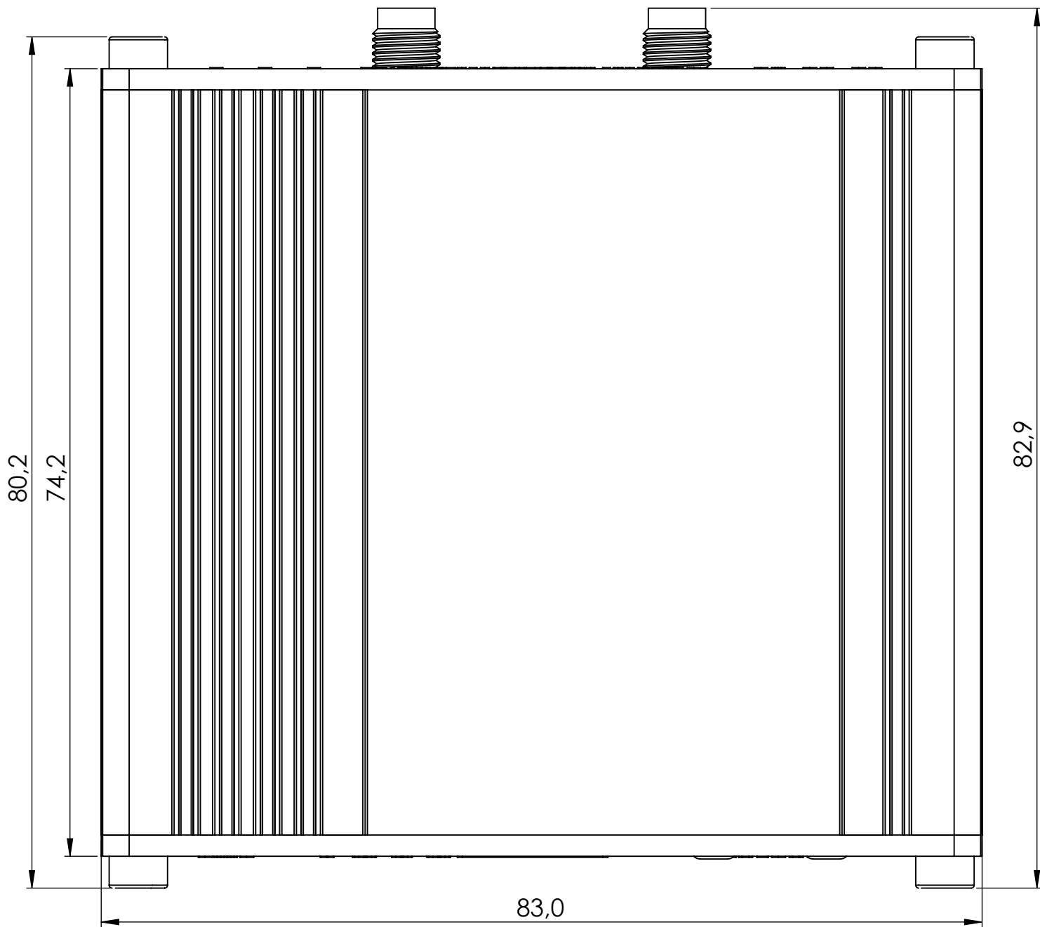
Top view
