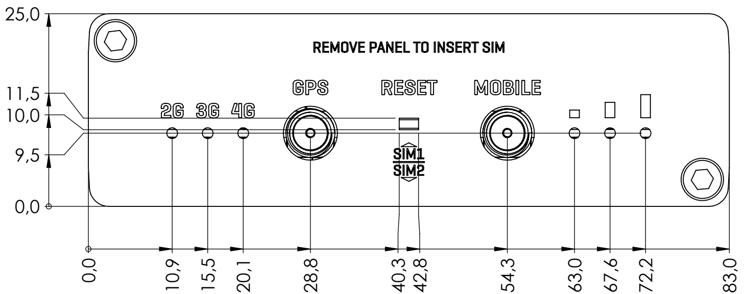
Rear view
