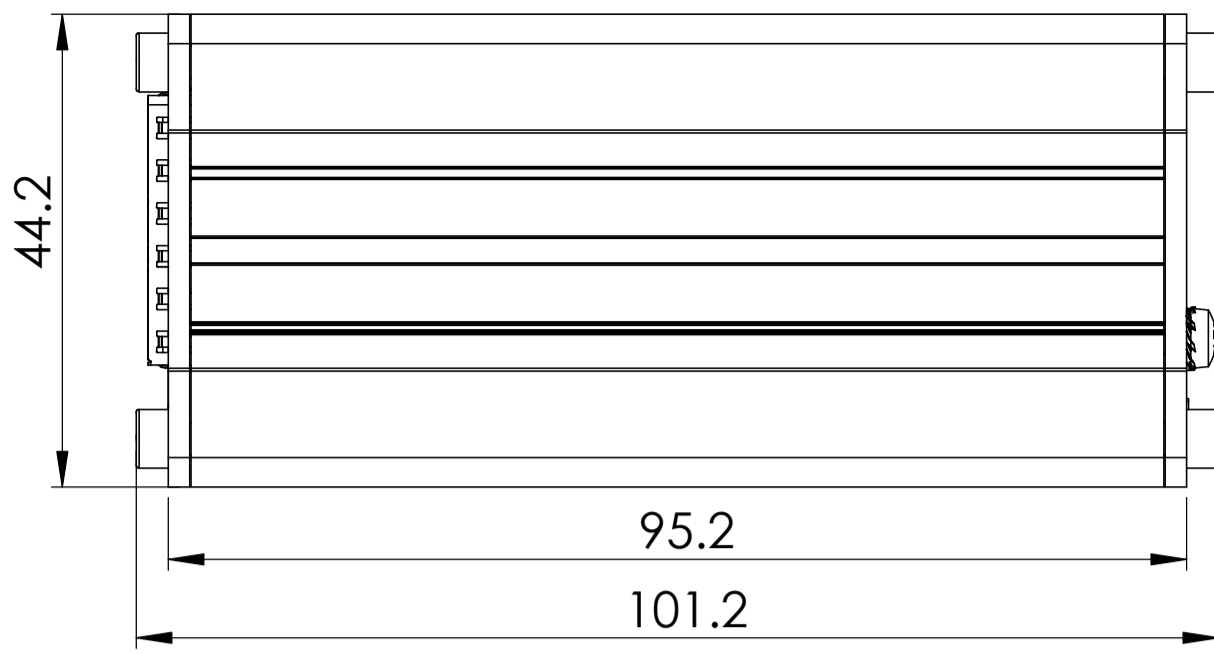
Right view
