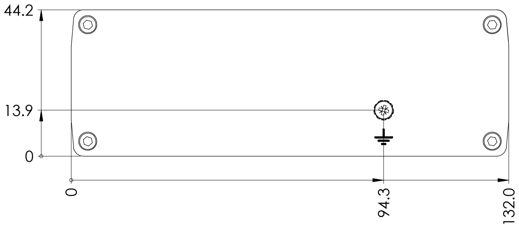
Rear view
