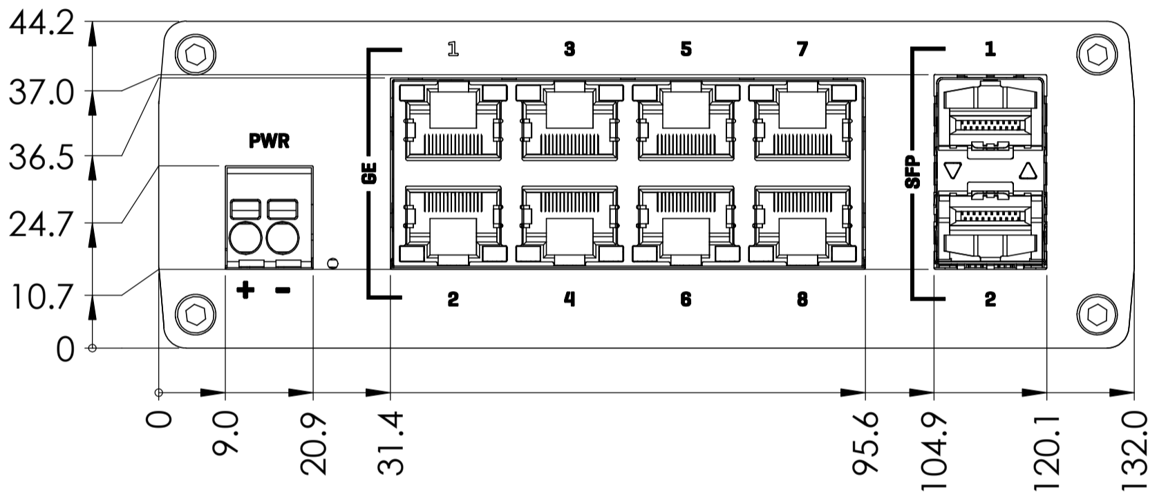
Front view
