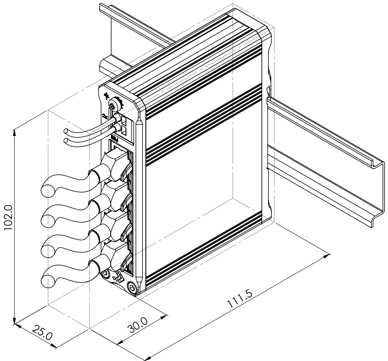
Mounting space requirements
