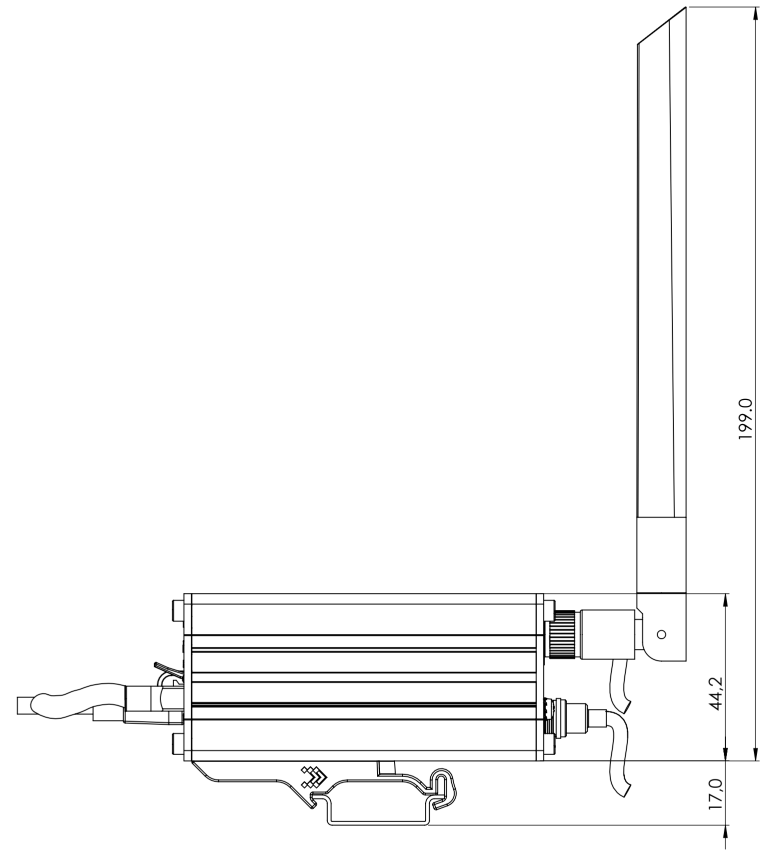
Mounting space requirements
