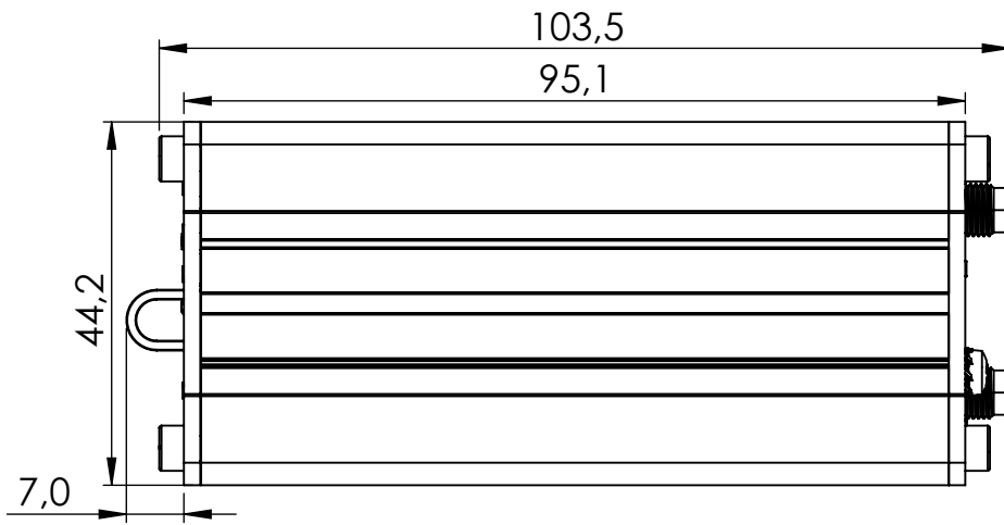
Right view
