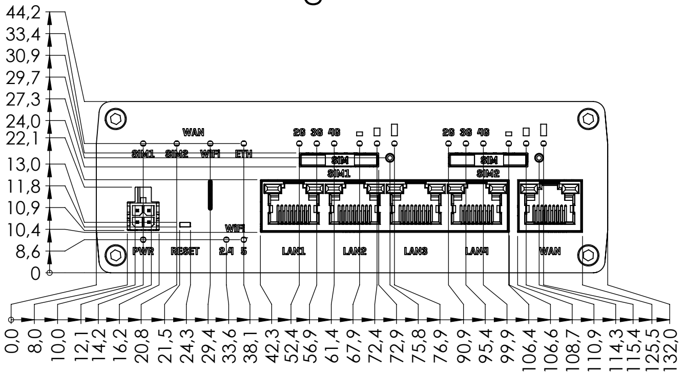
Right view
