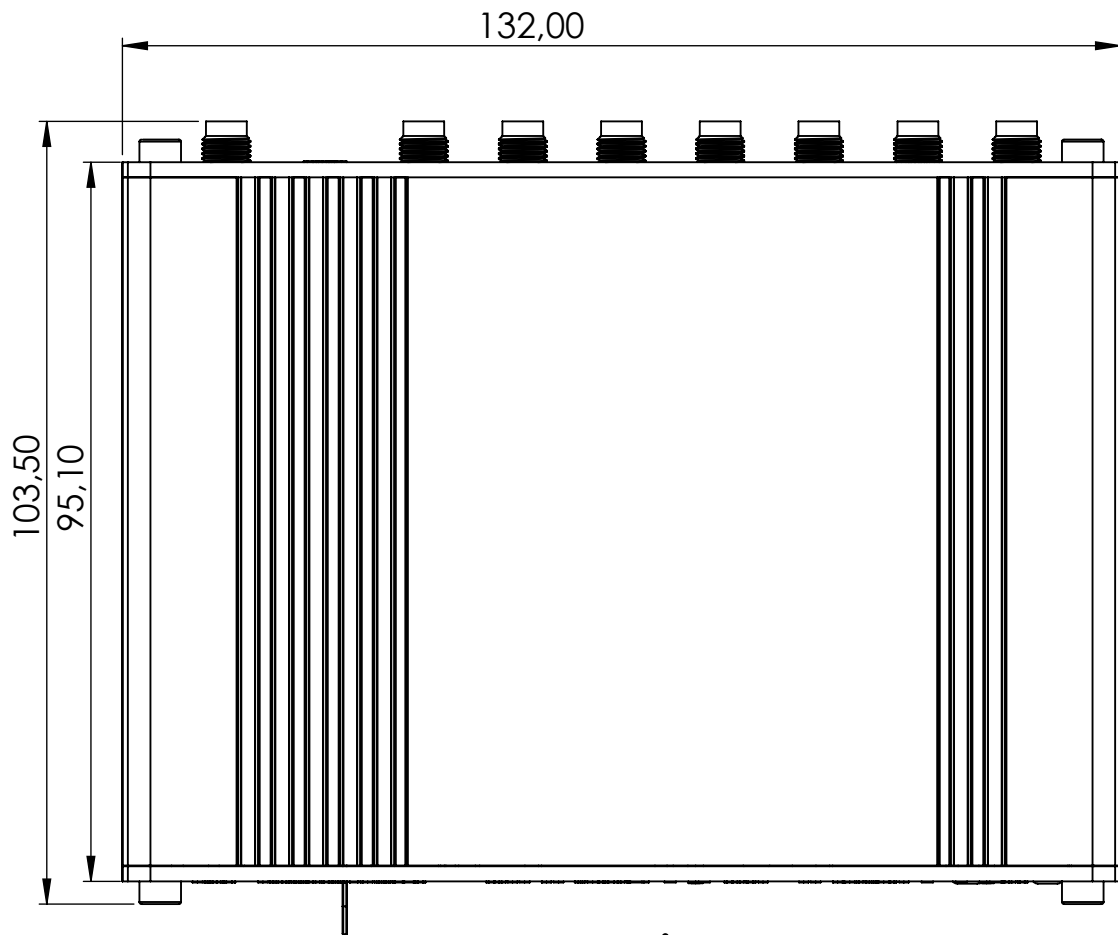
Top view
