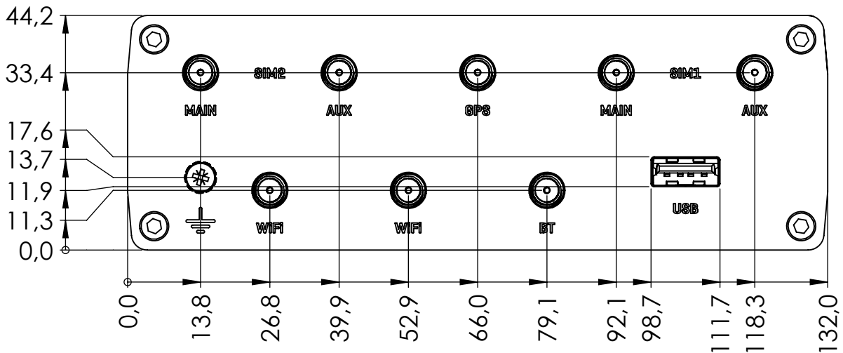
Rear view
