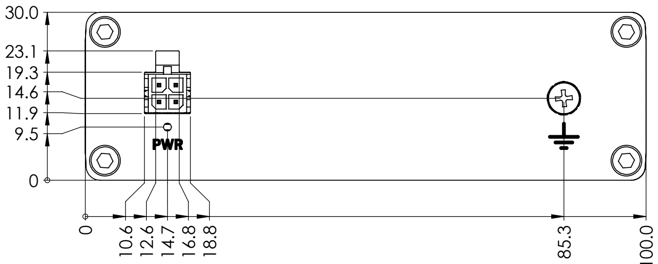
Rear view
