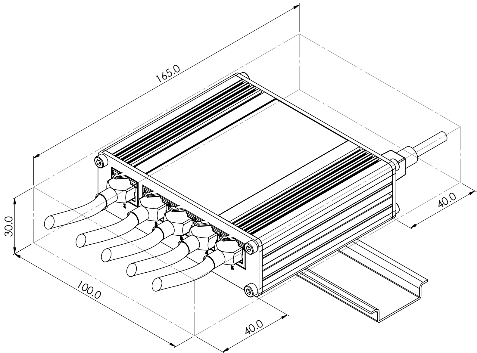
Mounting space requirements
