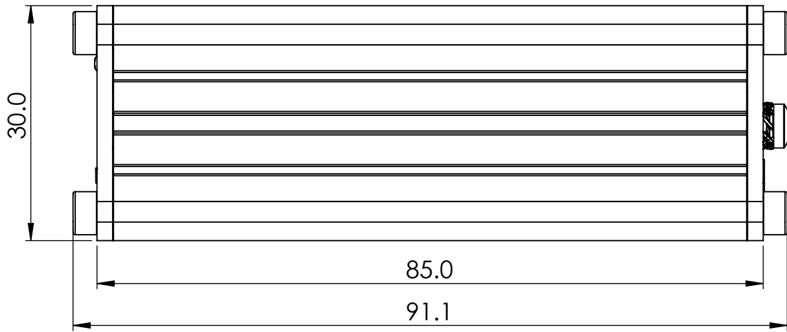
Right view
